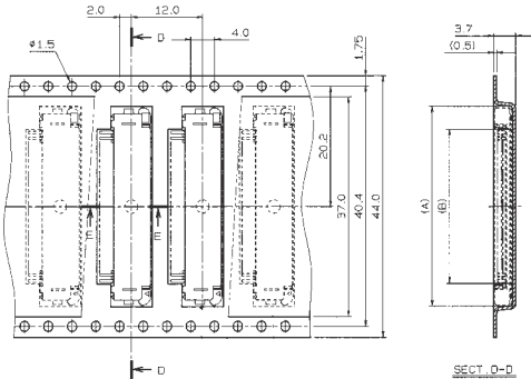
SECT. D-D
