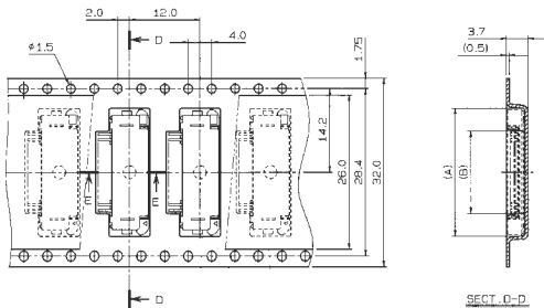
SECT. D-D
