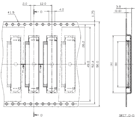
SECT. D-D
