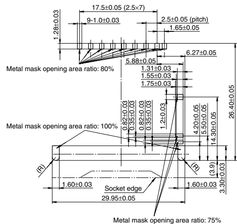
Recommended metal mask pattern
