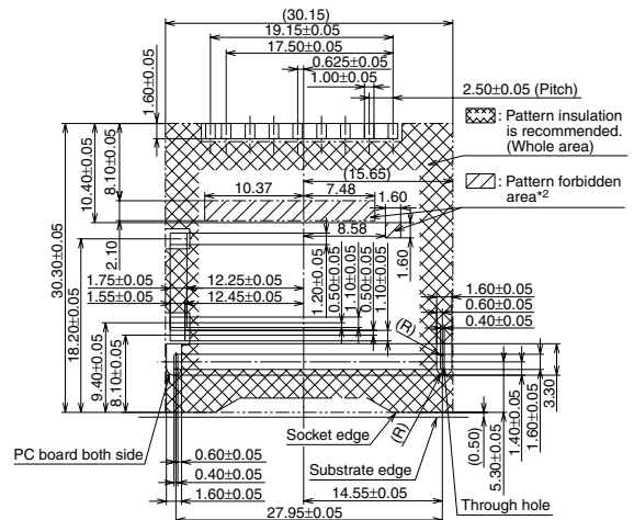
Recommended PC board pattern (TOP VIEW)
