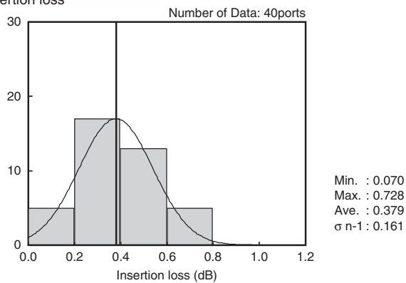
a) Insertion loss
