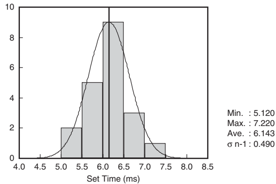
a) Set time
