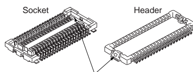
Locking structure of the retention fittings
