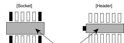
Pattern wiring under the connector is possible.
