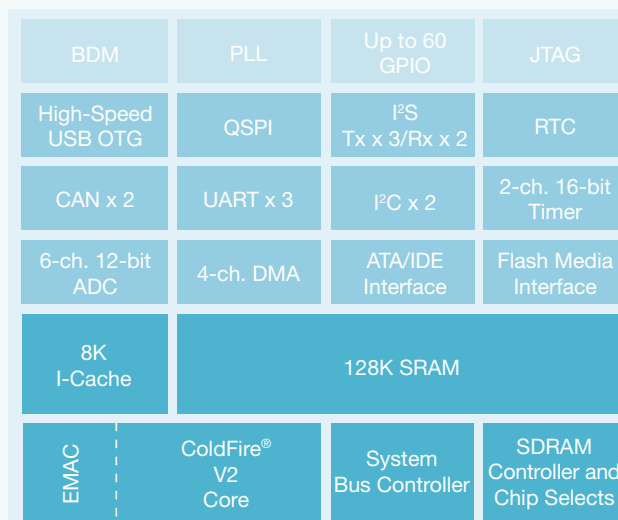
MCF5253 Block Diagram
