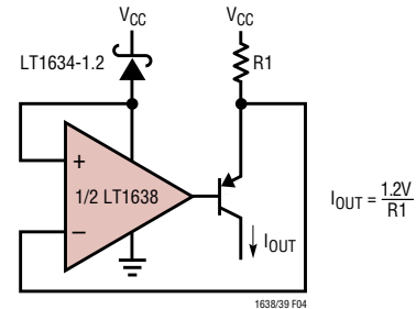
Figure 4. Current Source
